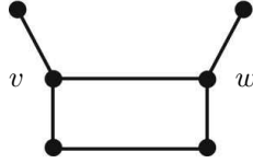
FIGURE 3. \Gamma_0 = [v, w]
