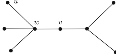
FIGURE 4. \Gamma - st(v) has more components than \Gamma - \{v\}
