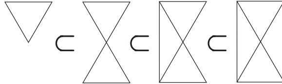
Figure 6: \Phi(\Theta_3) in the bordified chain complex.
