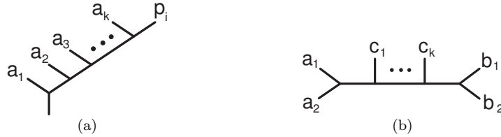
Figure 1: (a) The unique tree on which \mathfrak{D}_{p_i} does not vanish, and (b) an element of \mathcal{L}\mathcal{L}_n(k+2) .
