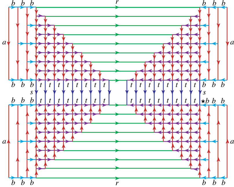
F 3. The van Kampen diagram \hat{\Delta}_3 for w_3 .
