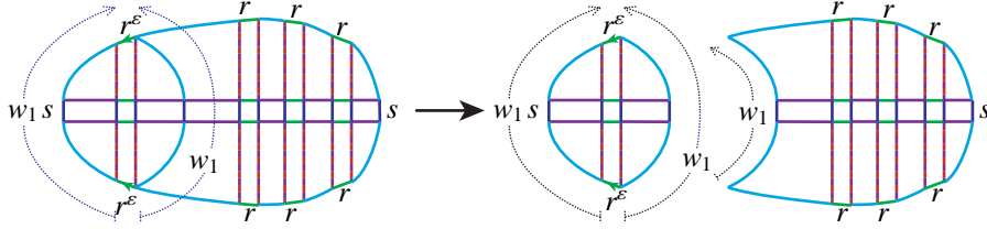
F 9. Shelling away one r -corridor.
