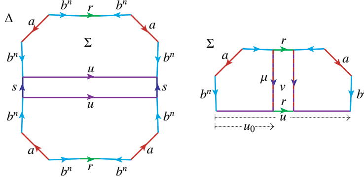
F 2. A van Kampen diagram \Delta for w_n with a subdiagram \Sigma .
