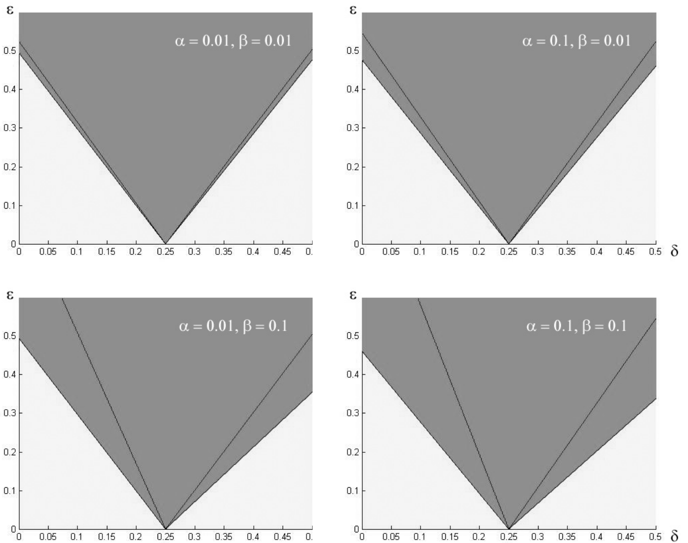
Figure 2: Shaded regions are unstable, unshaded regions are stable.
