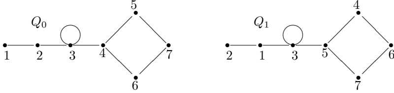
Figure 3. A seven-point example
