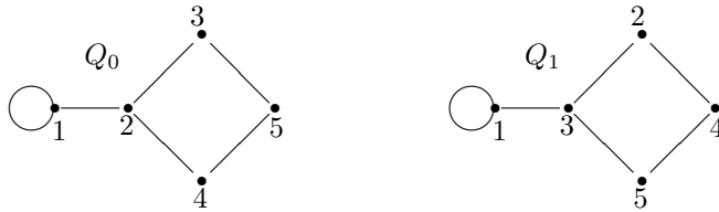
Figure 2. A five-point example
