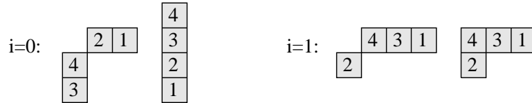
Figure 5: The tableaux contributing to H^i(\mathcal{M}_{\mathcal{A}}; k) .
