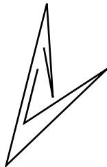
Figure 1: A polygonal chain in the plane.
