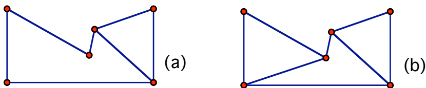
Figure 12: An edge is added to the graph of part (a) to get the graph of part (b), such that all the vertices remain pointed.
