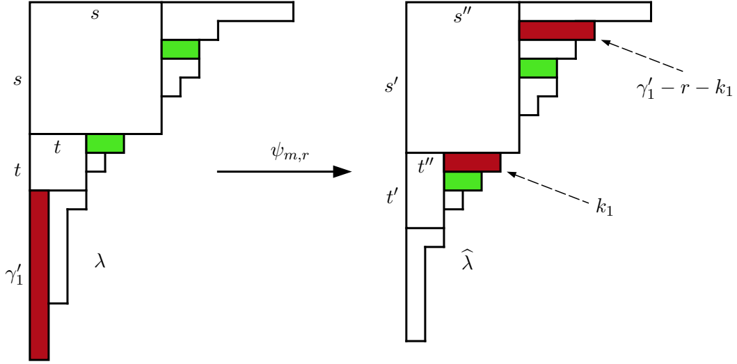
FIGURE 5. An example of the second symmetry bijection \psi_{m,r} : \lambda \mapsto \hat{\lambda} , where \lambda \in \mathcal{H}_{n,m,\leq -r} , \hat{\lambda} \in \mathcal{H}_{n',m+2,\geq -r} , for m = 0 , r = 2 , n = 92 , and n' = n - r - 2m - 2 = 88 . Here r_{2,0}(\lambda) = 2 + 2 - 9 = -5 \leq -2 and r_{2,2}(\hat{\lambda}) = 3 + 4 - 6 = 1 \geq -2 , where \lambda = (14, 10, 9, 9, 8, 7, 7, 5, 4, 3, 3, 2, 2, 2, 2, 1, 1, 1) and \hat{\lambda} = (13, 10, 9, 8, 8, 7, 6, 6, 5, 4, 3, 2, 2, 1, 1, 1, 1, 1) . Also, s = 7 , s' = s + 1 = 8 , s'' = s' - m - 2 = 6 , t = 3 , t' = 4 , t'' = 2 , \gamma'_1 = 9 , k_1 = 3 , and \gamma'_1 - r - k_1 = 4 .
